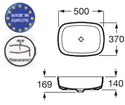
Inspira 柔方形枱上盆* A327500630
