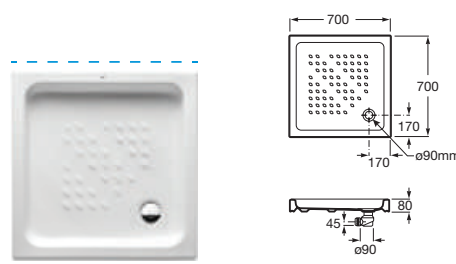
Italia Square 陶瓷淋浴盆 A3740HK000
