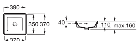
THE GAP SQUARE 半枱上盆
