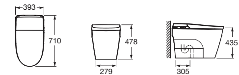
IN-WASH® INSPIRA FLOOR-STANDING 一體式智能座廁 A8030R2008 地排 305mm $30,160
