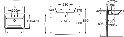
THE GAP 面盆 (掛牆·枱上盆兩用)
