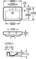
DAMA SENSO SQUARE 掛牆面盆
