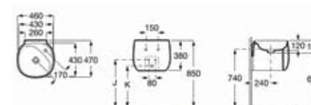
BEYOND 掛牆面盆
