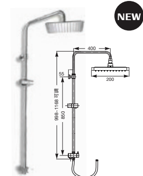
RAINSENSE MOVABLE 方形淋浴柱 (200x200mm) (可調校高度)
