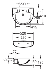
DAMA SENSO SQUARE 掛牆面盆
