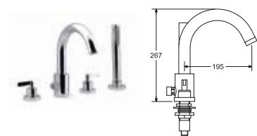
ATTIC 座枱浴缸龍頭連花灑
