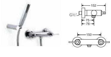
ATTIC 淋浴龍頭連花灑
